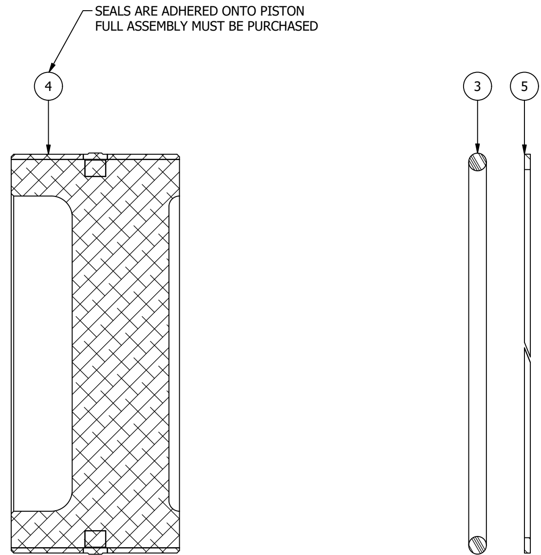
SECTION VIEW
