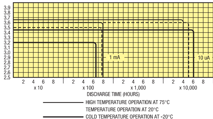
TYPICAL LTC-7PN DISCHARGE CHARACTERISTICS AT VARIED TEMPERATURES
