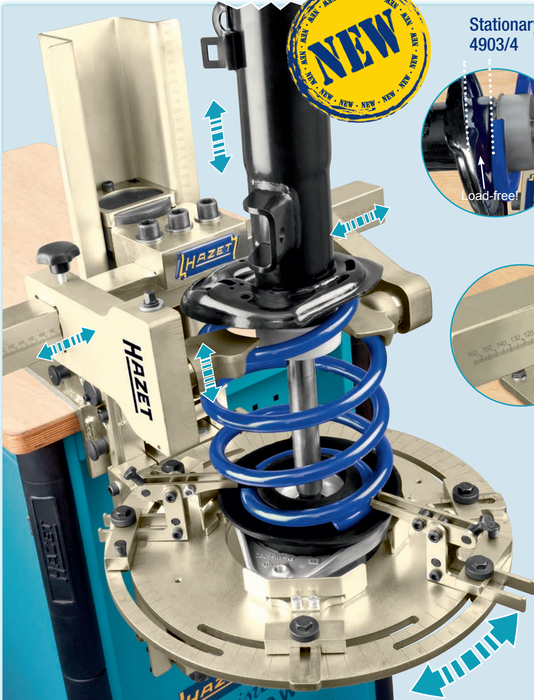
Spring Vice 4903/4
