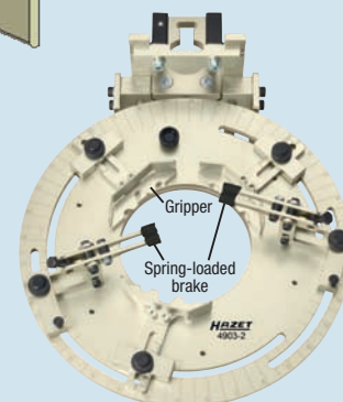
4903-2 Clamping disc (adjustable)
