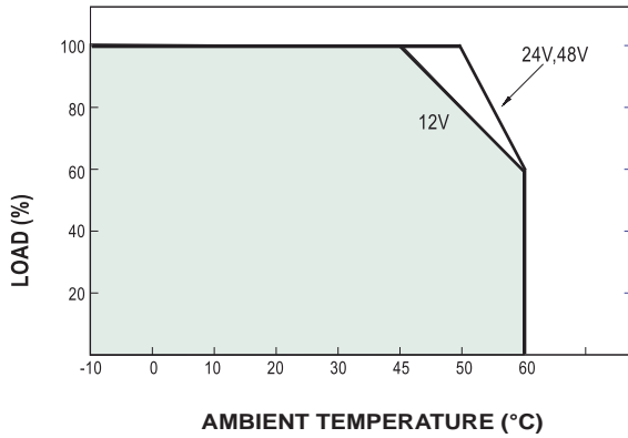
Output Derating :
